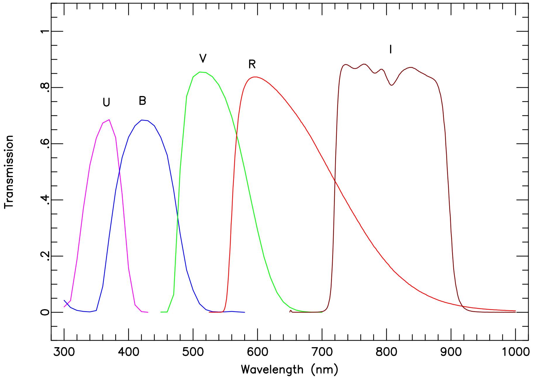
OSU 2.5" UBVRI Filter Transmission Curves
